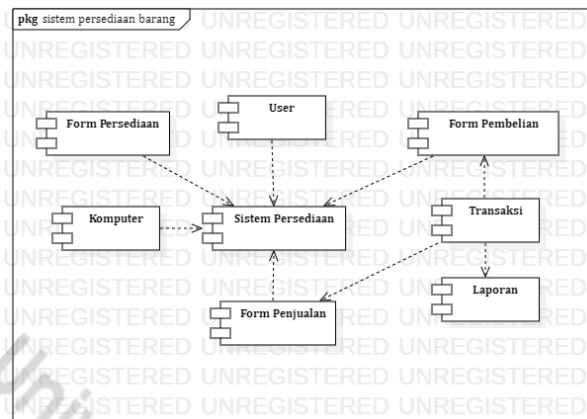
Gambar 6. Component Diagram Sistem Persediaan
