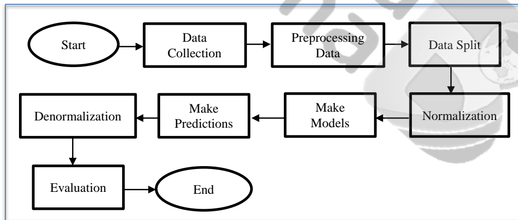
Figure 1. Research Flowchart
