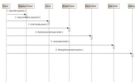
Gambar Sequence Deployment Diagram
