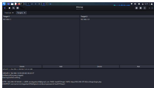
Figure 7. Man-in-the-Middle attack
