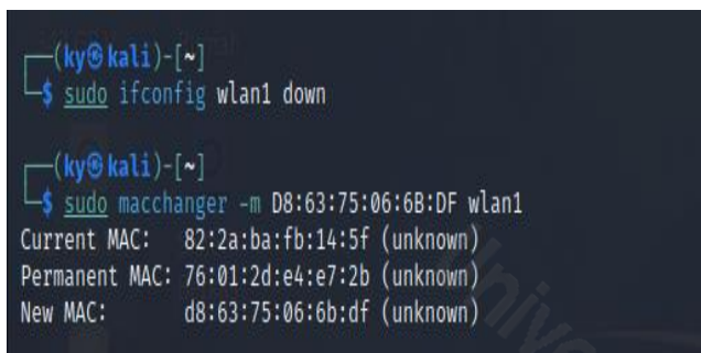
Figure 6. MAC Spoofing
