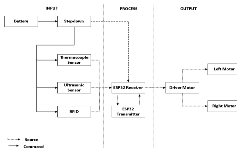
Figure 4 Receiver Block Diagram
