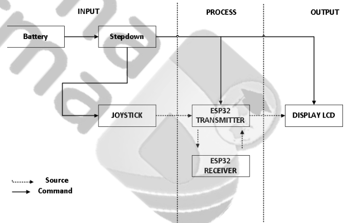
Figure 3 Block Transmitter Diagram
