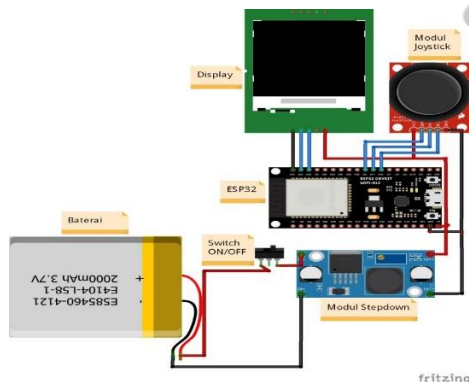
Figure 1 Schematic Circuit on Device Transmitter
