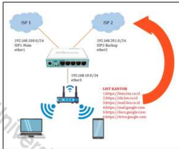
Figure 3 Policy Based Route schema
