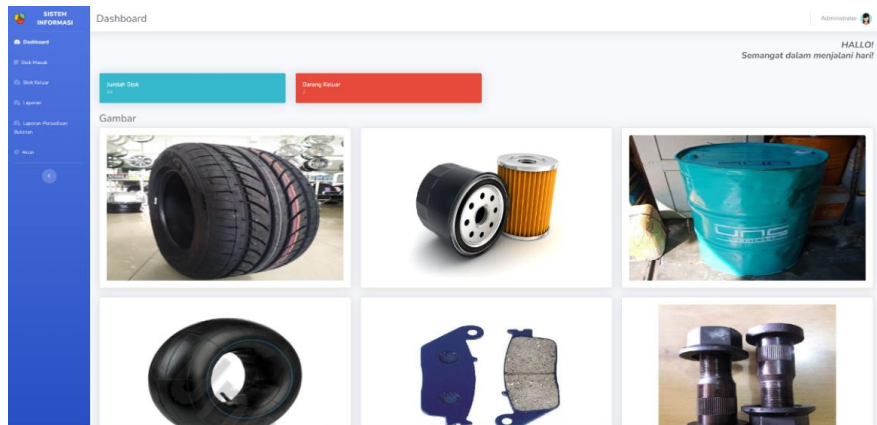
Gambar 4.2 Tampilan dashboard
