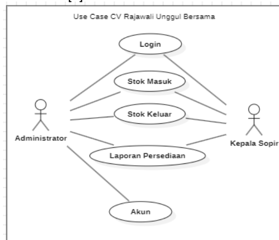
Gambar 2.1 Use Case Diagram
