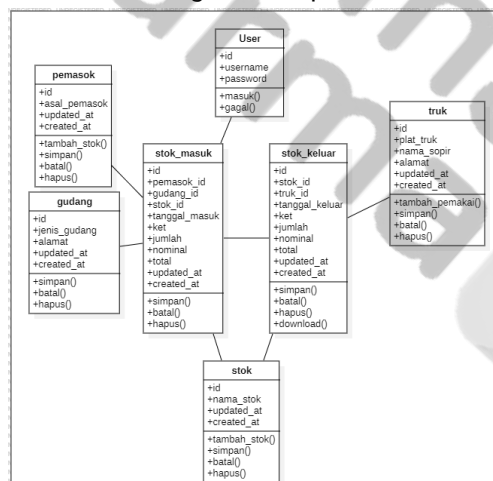
Gambar 2.3 Class Diagram
