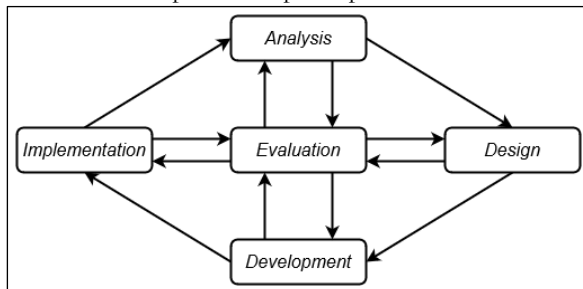
Gambar 1. Metode ADDIE
